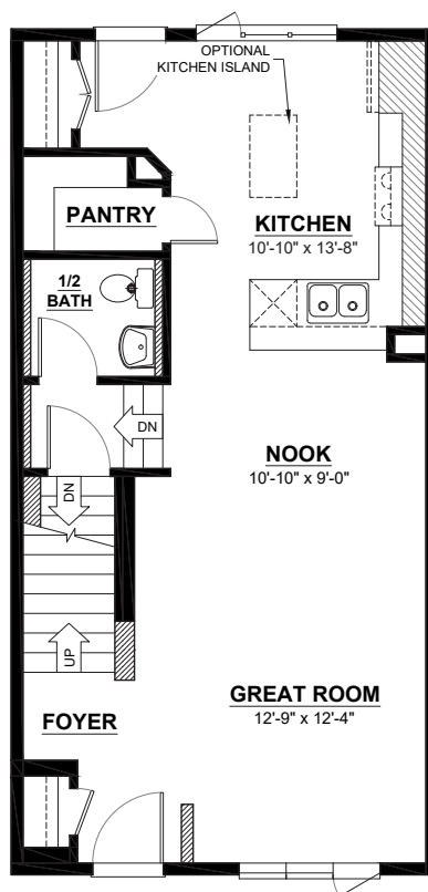
MAIN FLOOR 648 Sq. Ft. | 8 Ft. ceiling
