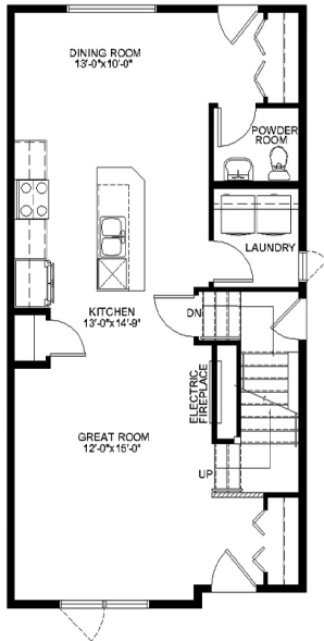
MAIN FLOOR AREA: 773 SQ. FT.
